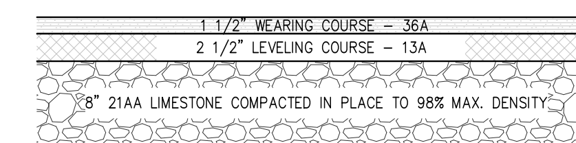
STANDARD ASPHALT PAVE CROSS-SECTION
