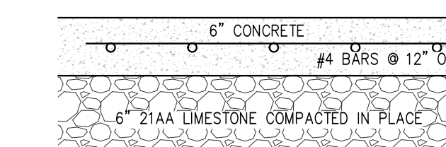
STANDARD CONCRETE PAVE CROSS-SECTION
