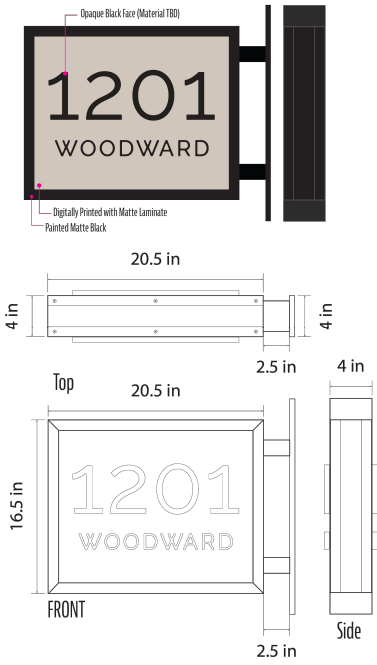
EXTERIOR ADDRESS SIGNAGE DETAIL NOT TO SCALE
