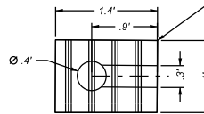
BUILDING MOUNTED, LIGHTING (QTY 4) 1.4' X 1.0' 0' TO 13' ABOVE GRADE
