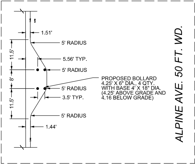
BOLLARD DETAIL
