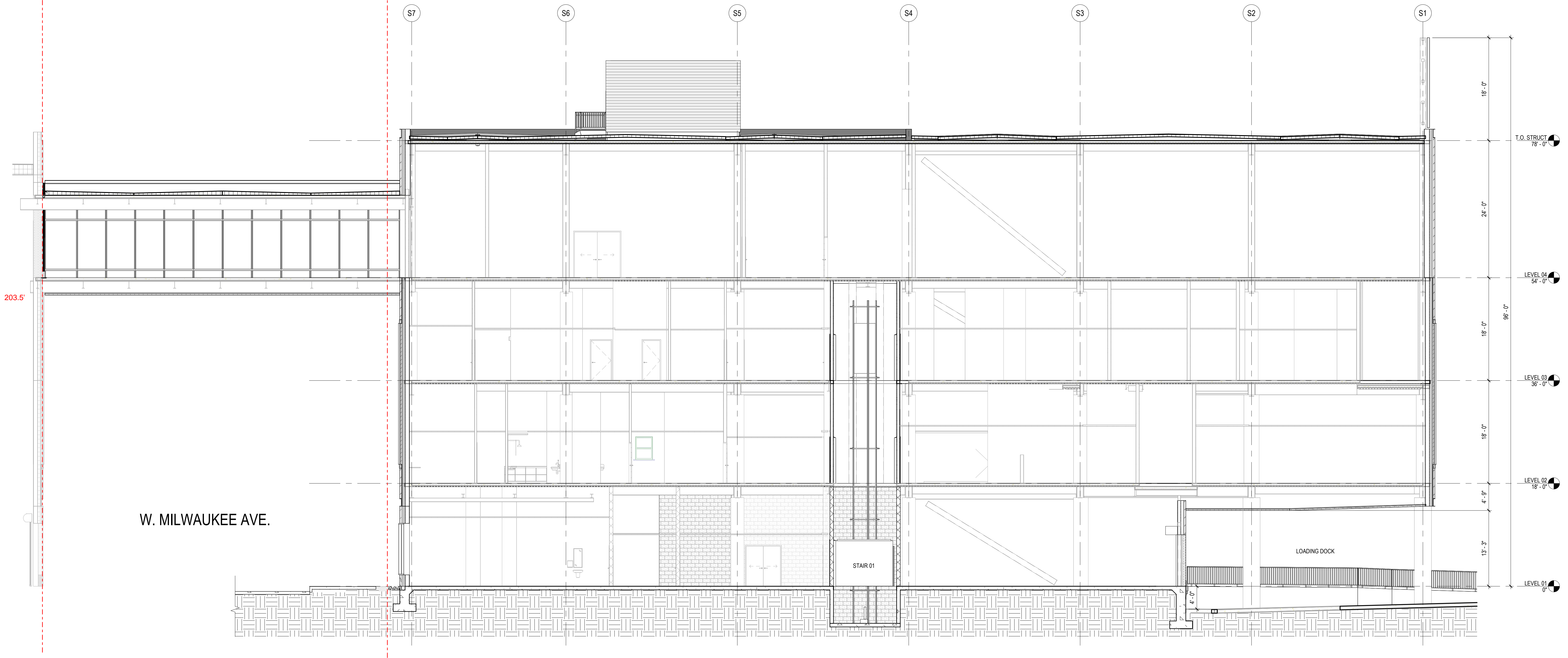
C5 BUILDING SECTION 4 1/8" = 1'-0"
