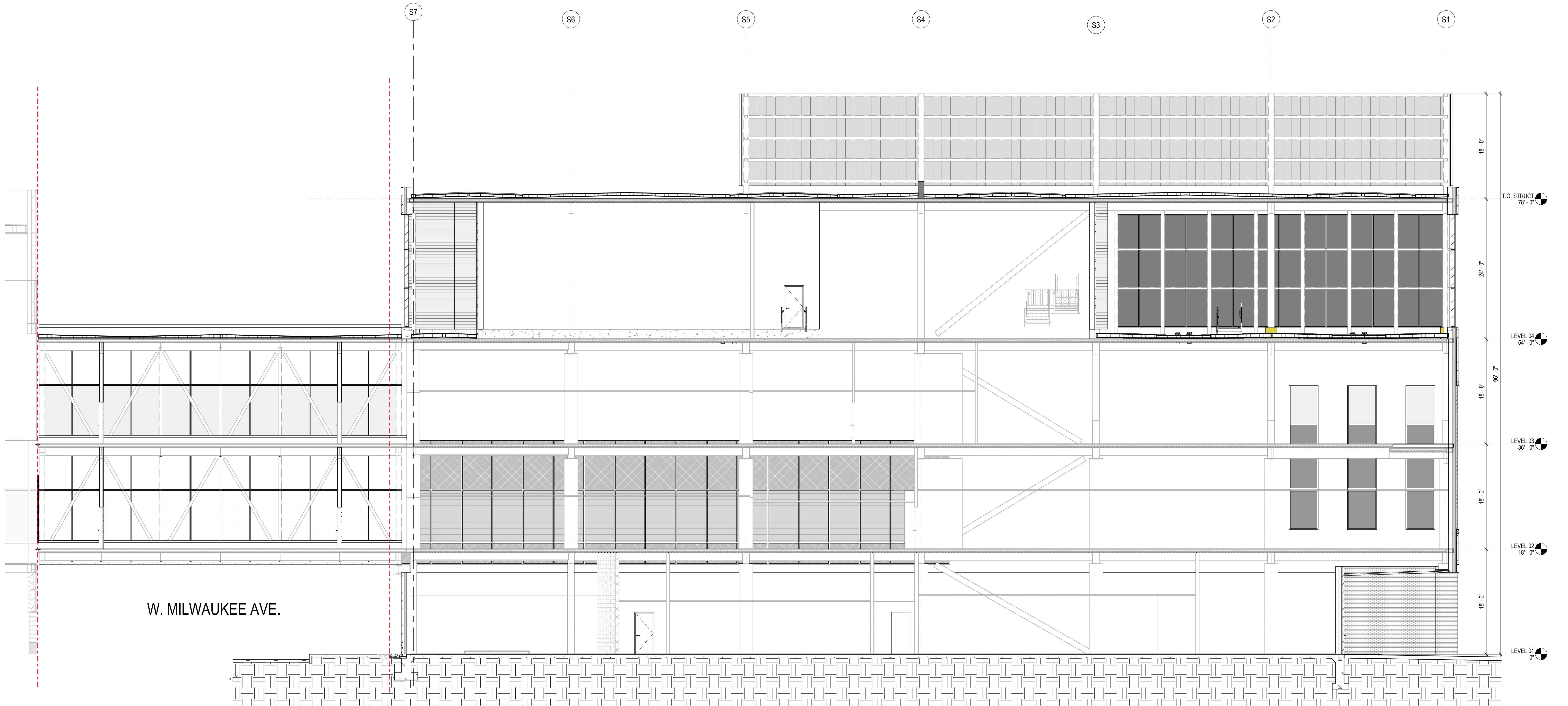
C5 BUILDING SECTION 2 1/8" = 1'-0"
