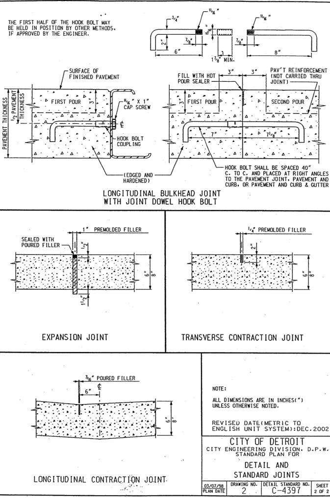
07 DETAIL AND STANDARD JOINTS - CITY OF DETROIT NOT TO SCALE
