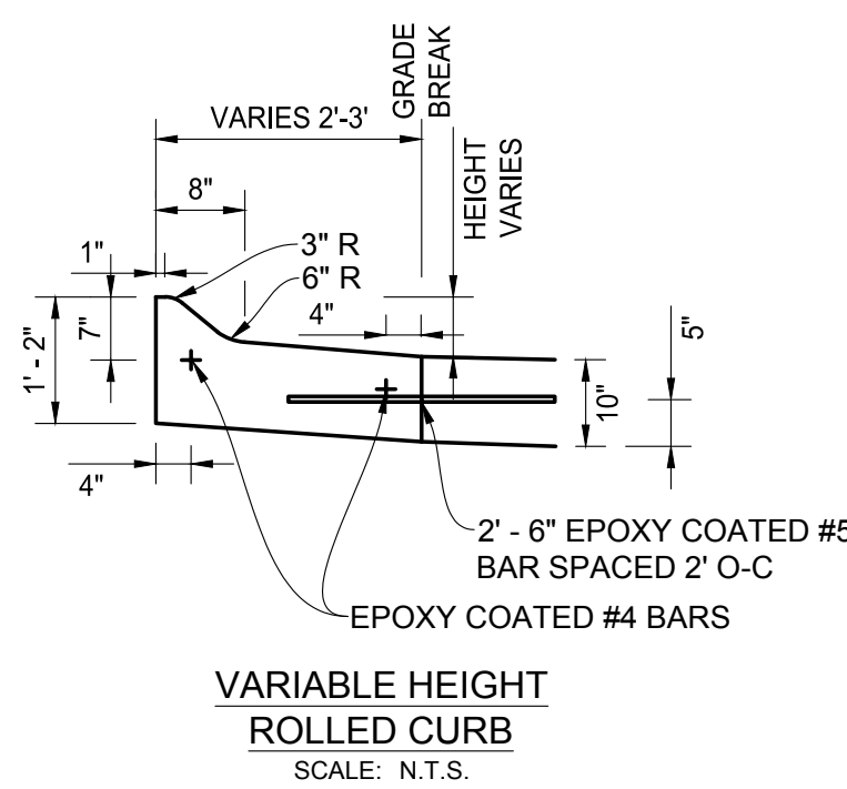
09 VARIABLE HEIGHT ROLLED CURB NOT TO SCALE
