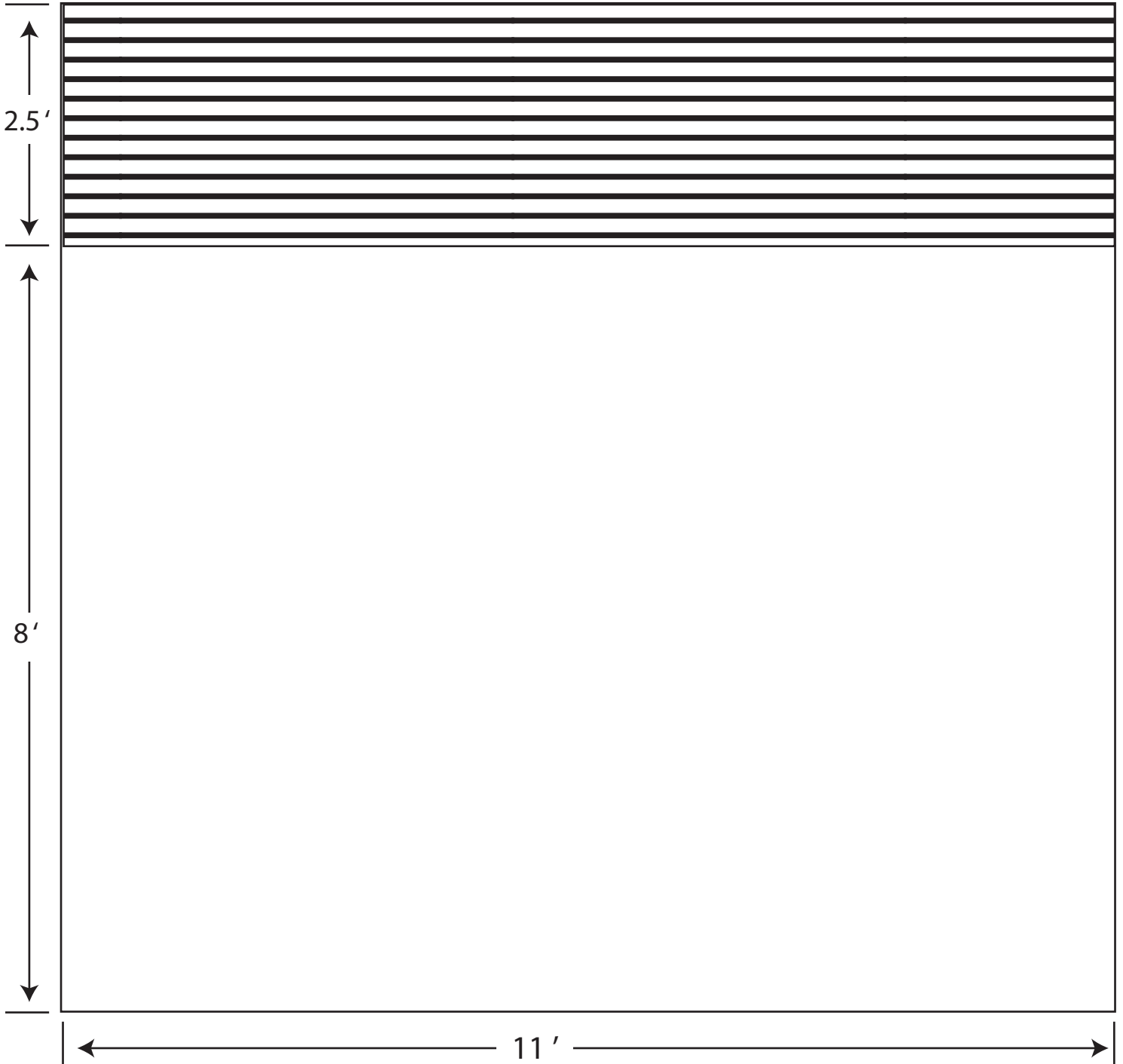
MEDIUM AWNING 11'W X 2.5'H x 2'D
