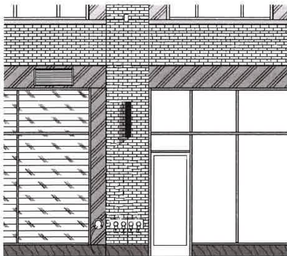
CONCEPT - 3/16" = 1'-0"
