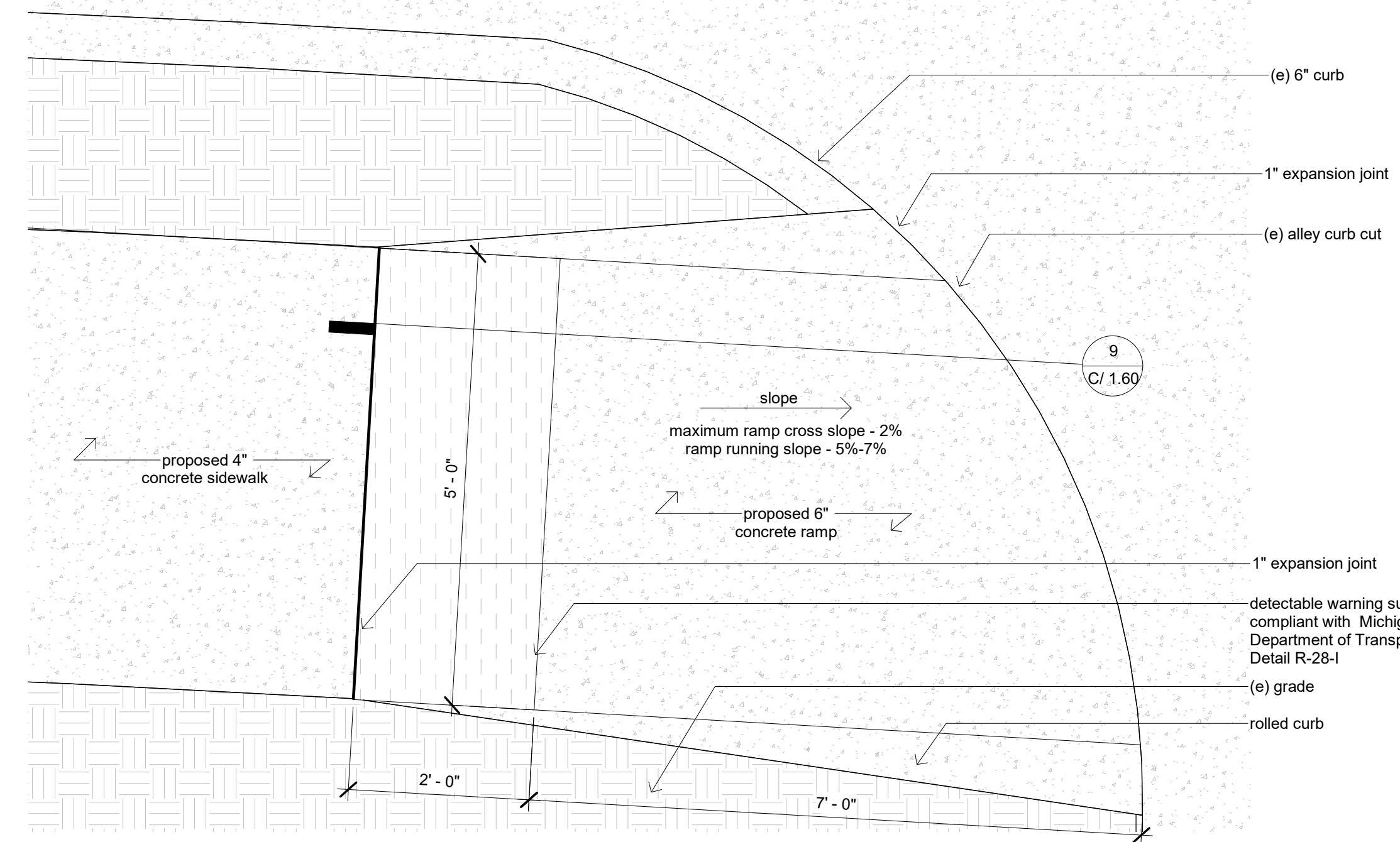
typical Type R curb cut 3/4" = 1'-0" 3
