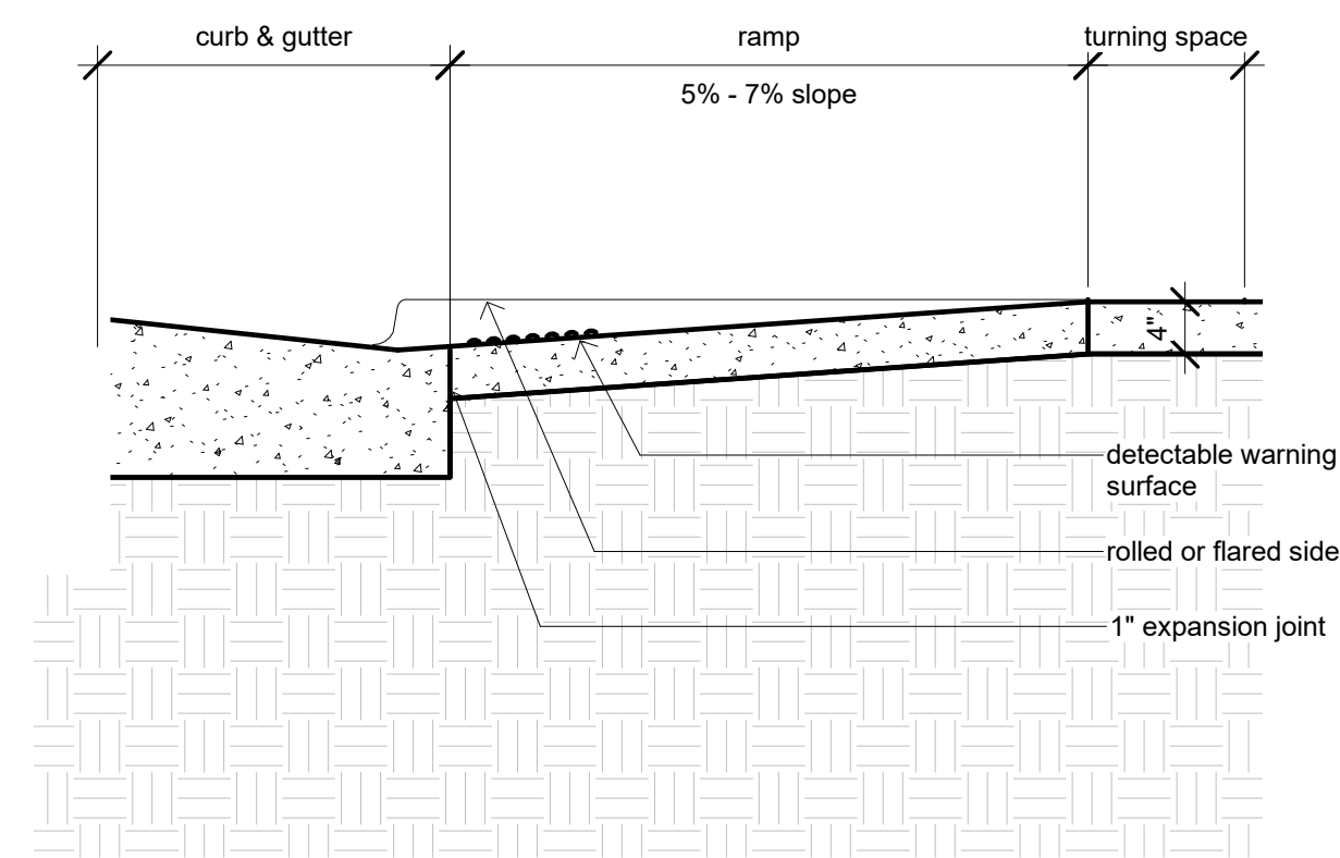
typical section / sidewalk ramp 3/4" = 1'-0" 9
