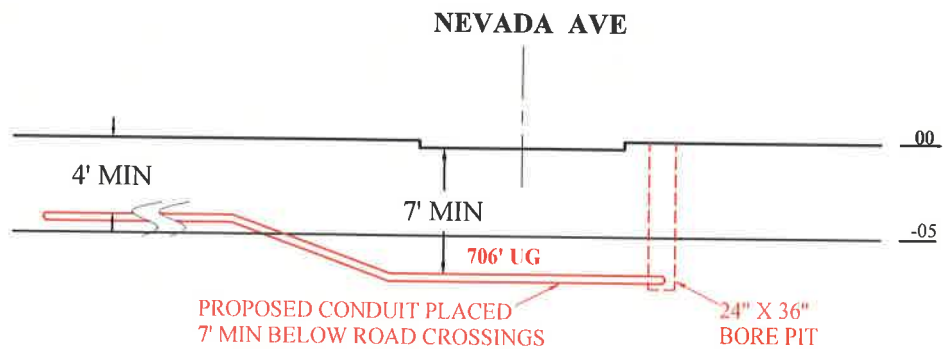
SECTION VIEW LOOKING WEST ALONG NEVADA AVE.
