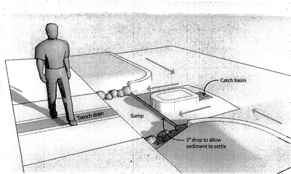
Hamilton Rain Garden Learning Lab INLET MODEL
