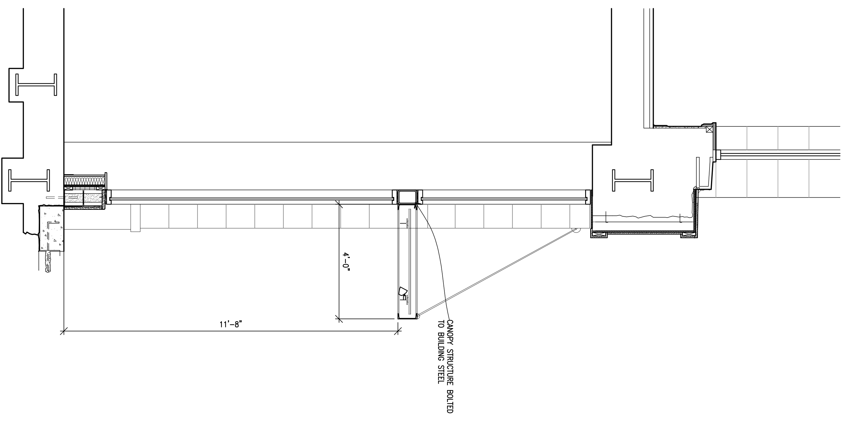
3 CLIFFORD SECTION VIEW SE-1 1/2" = 1'-0"
