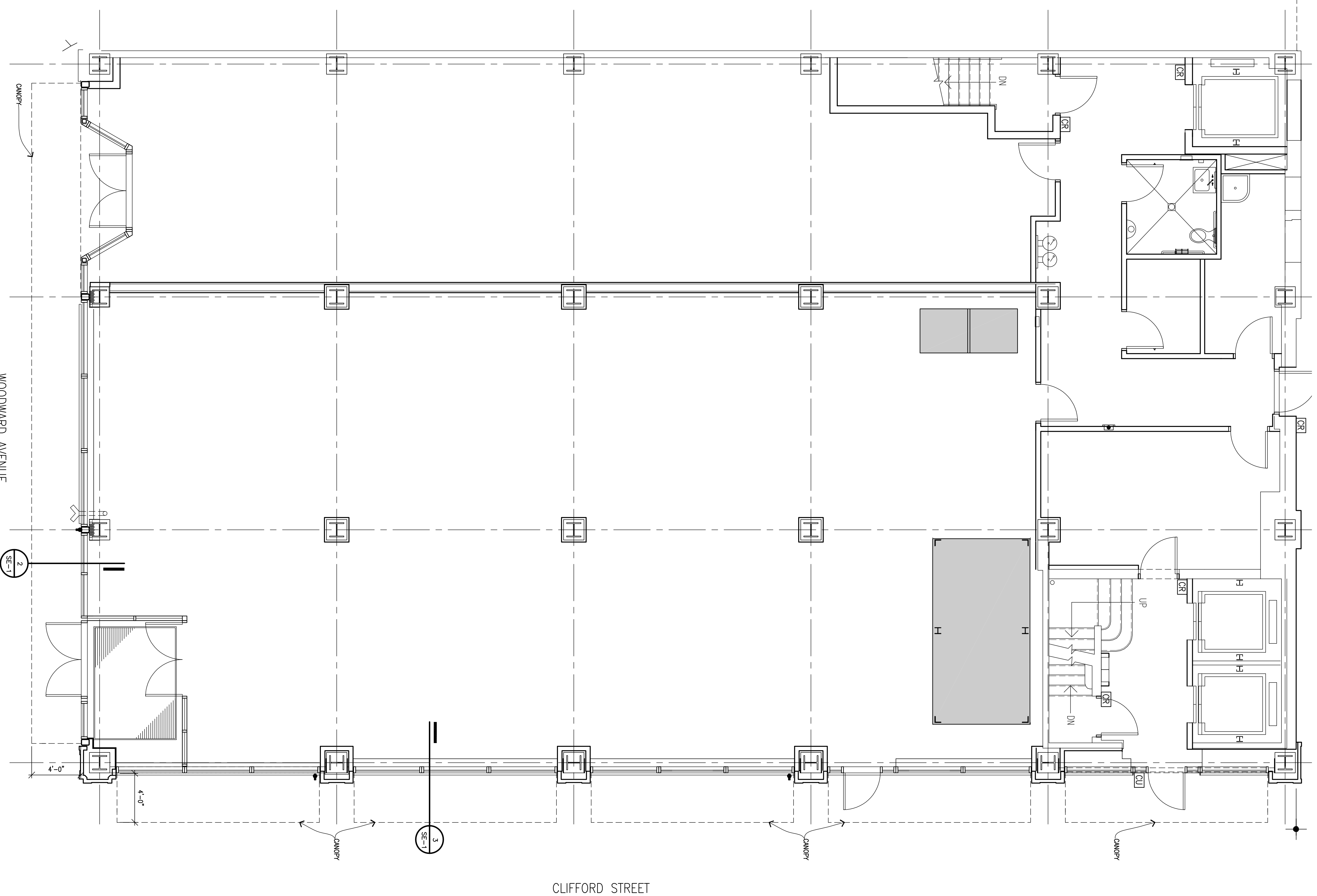
1 CANOPY ATTACHMENT LAYOUT SE-1 1/4" = 1'-0"
