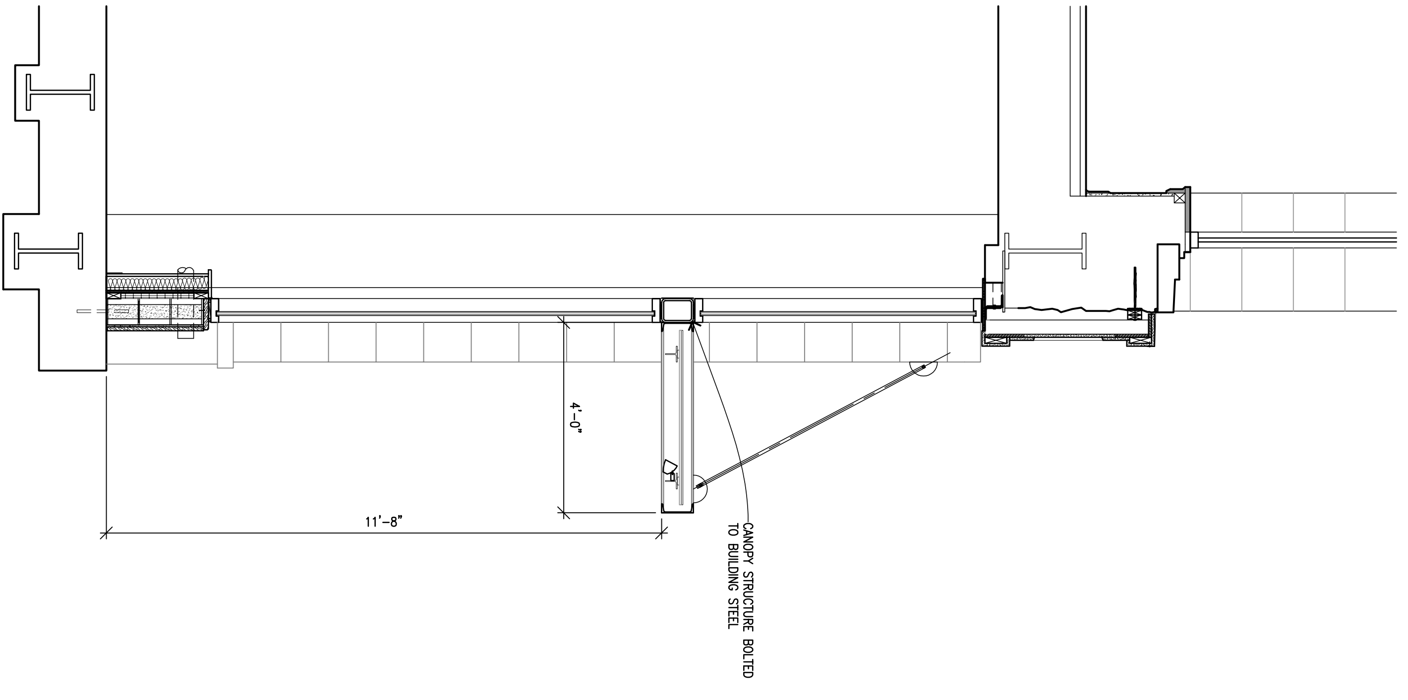
2 WOODWARD SECTION VIEW SE-1 1/2" = 1'-0"
