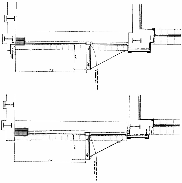
CLIFFORD SECTION VIEW
