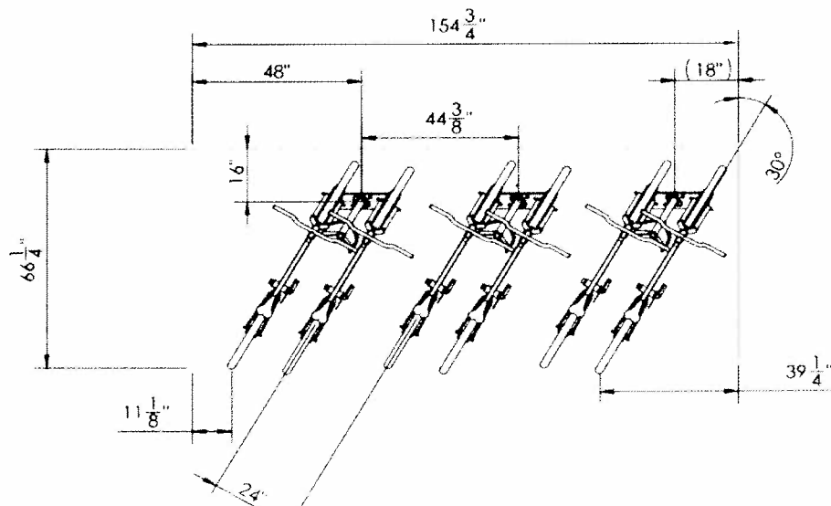
Bike rack Dimensions
