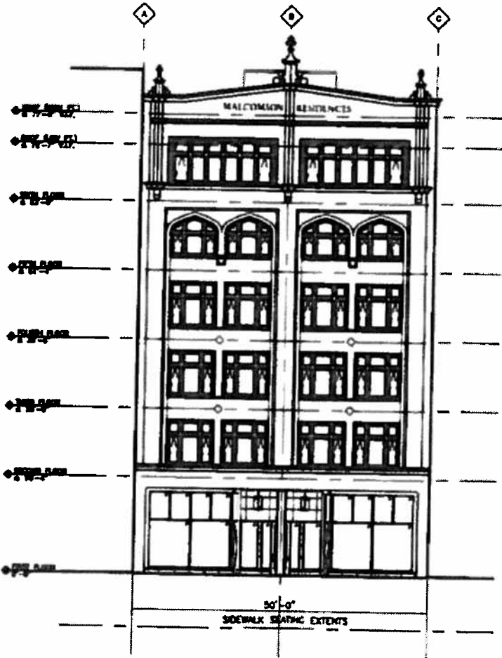
① EAST (GRISWOLD) ELEVATION SCALE: 1/16" = 1'-0"
