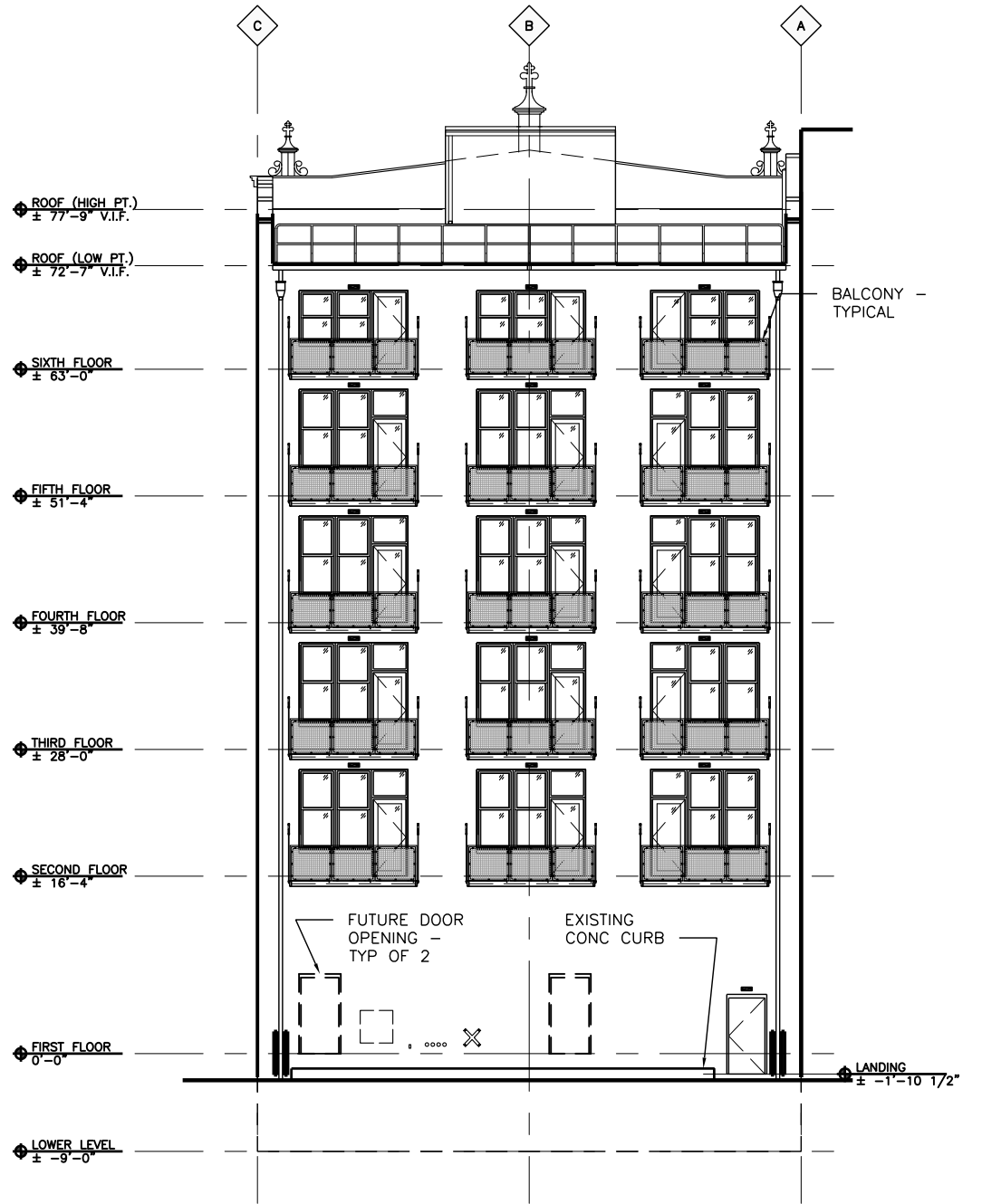
1 WEST (ALLEY) ELEVATION SCALE: 1/16" = 1'-0"
