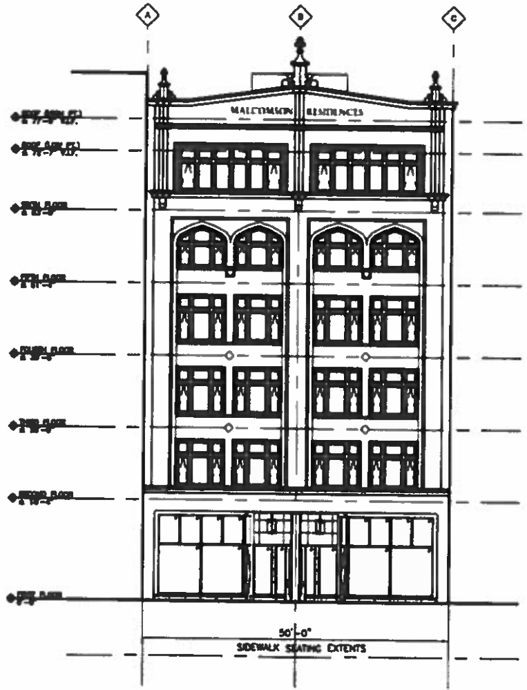
1 EAST (GRISWOLD) ELEVATION SCALE: 1/16" = 1'-0"
