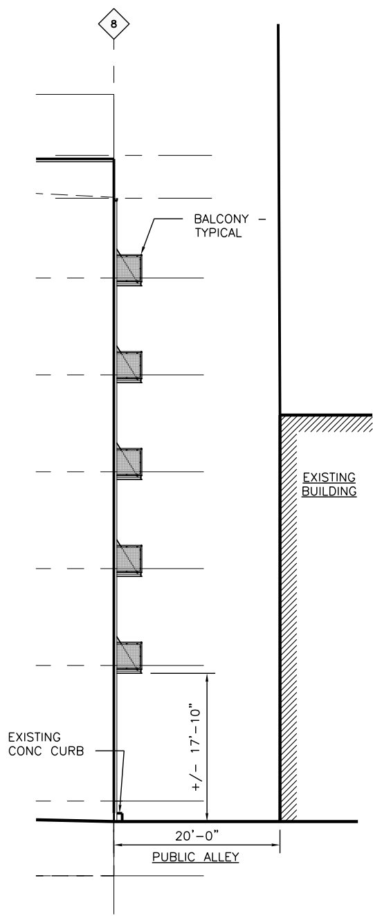
2 PARTIAL NORTH ELEVATION SCALE: 1/16" = 1'-0"
