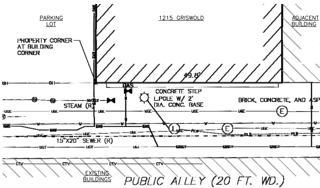
PARTIAL TOPOGRAPHIC SURVEY AT ALLEY SCALE: 1/16" = 1'-0"
