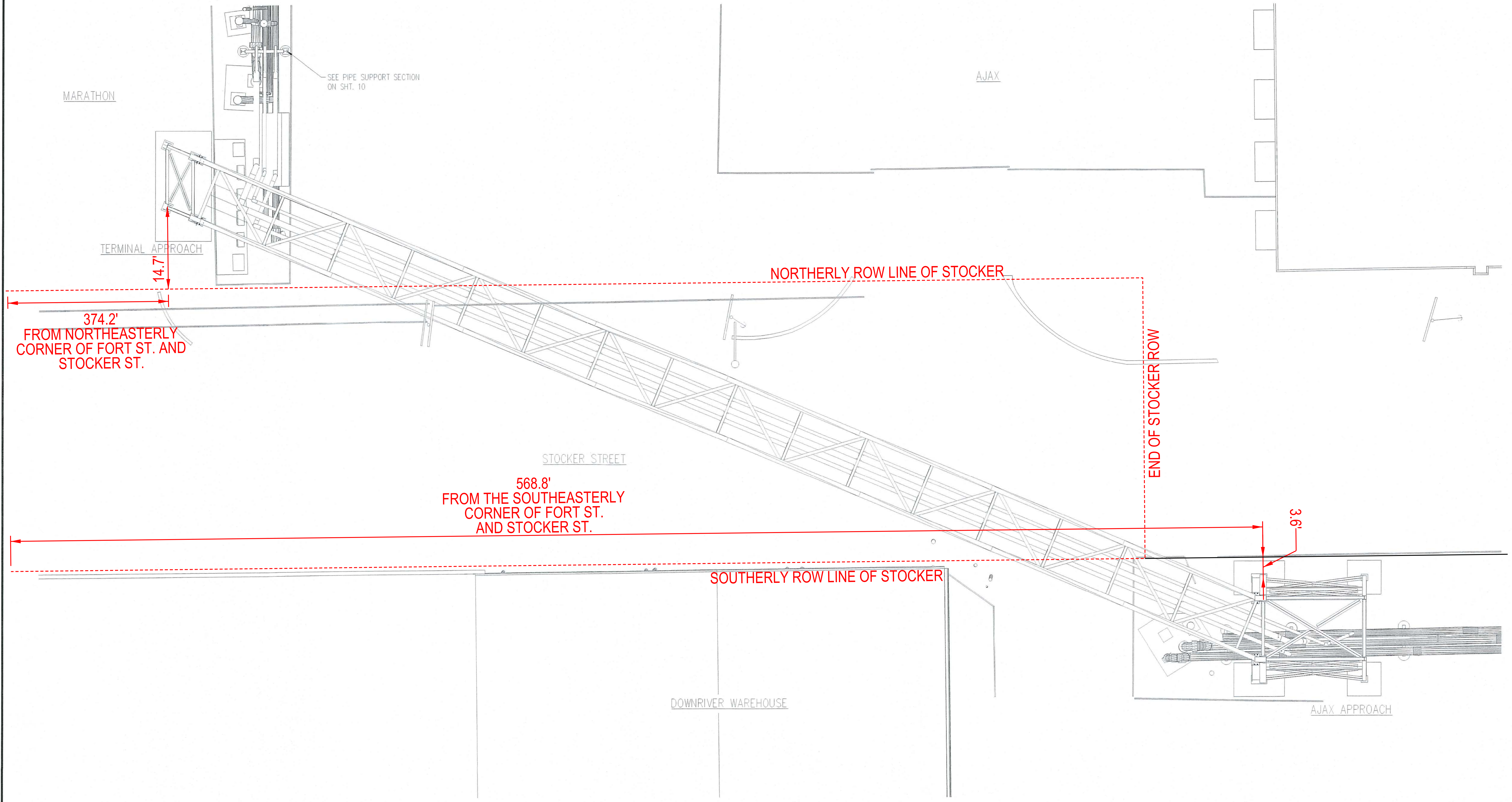
OVERALL PLAN SCALE: 1/8" = 1'-0"
