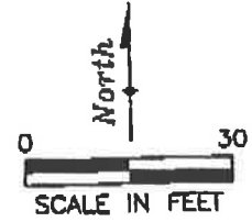
FIGURE 2.1 SITE MAP AMOCO SERVICE STATION NO. 5882 800 EAST SEVEN MILE ROAD DETROIT, MICHIGAN
