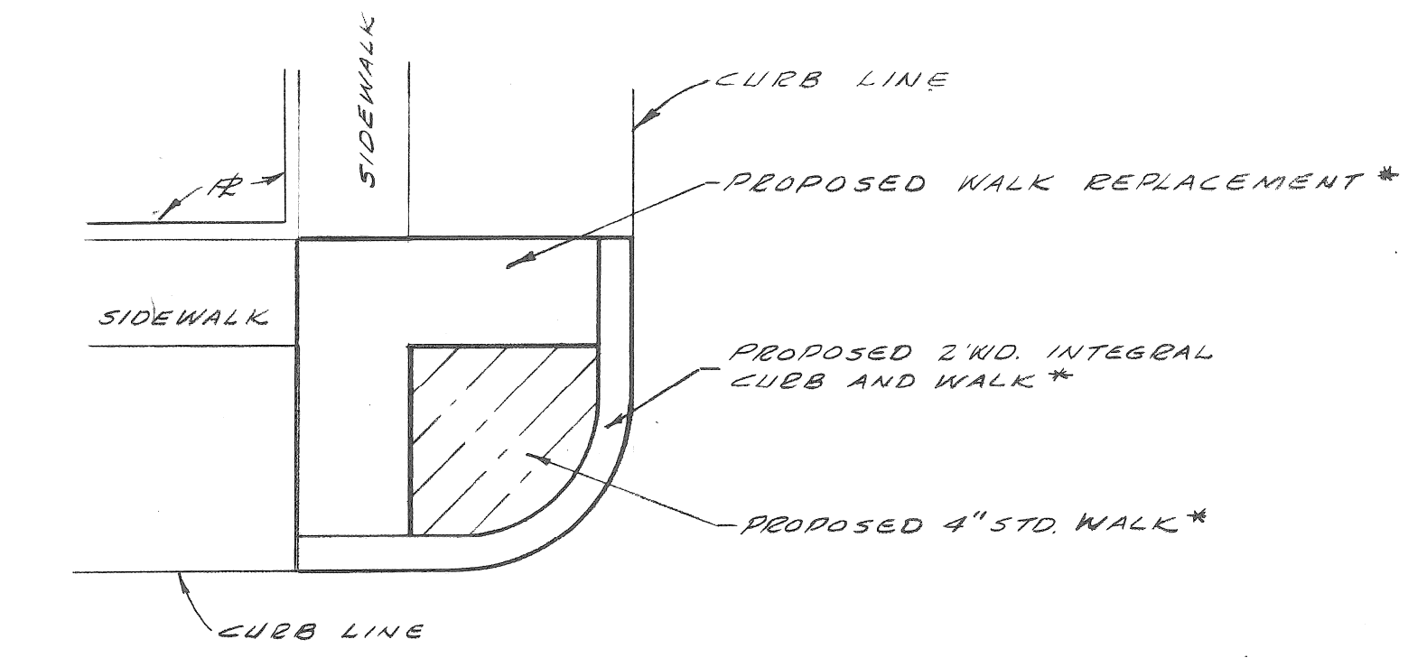
TYPICAL INTERSECTION NO SCALE
