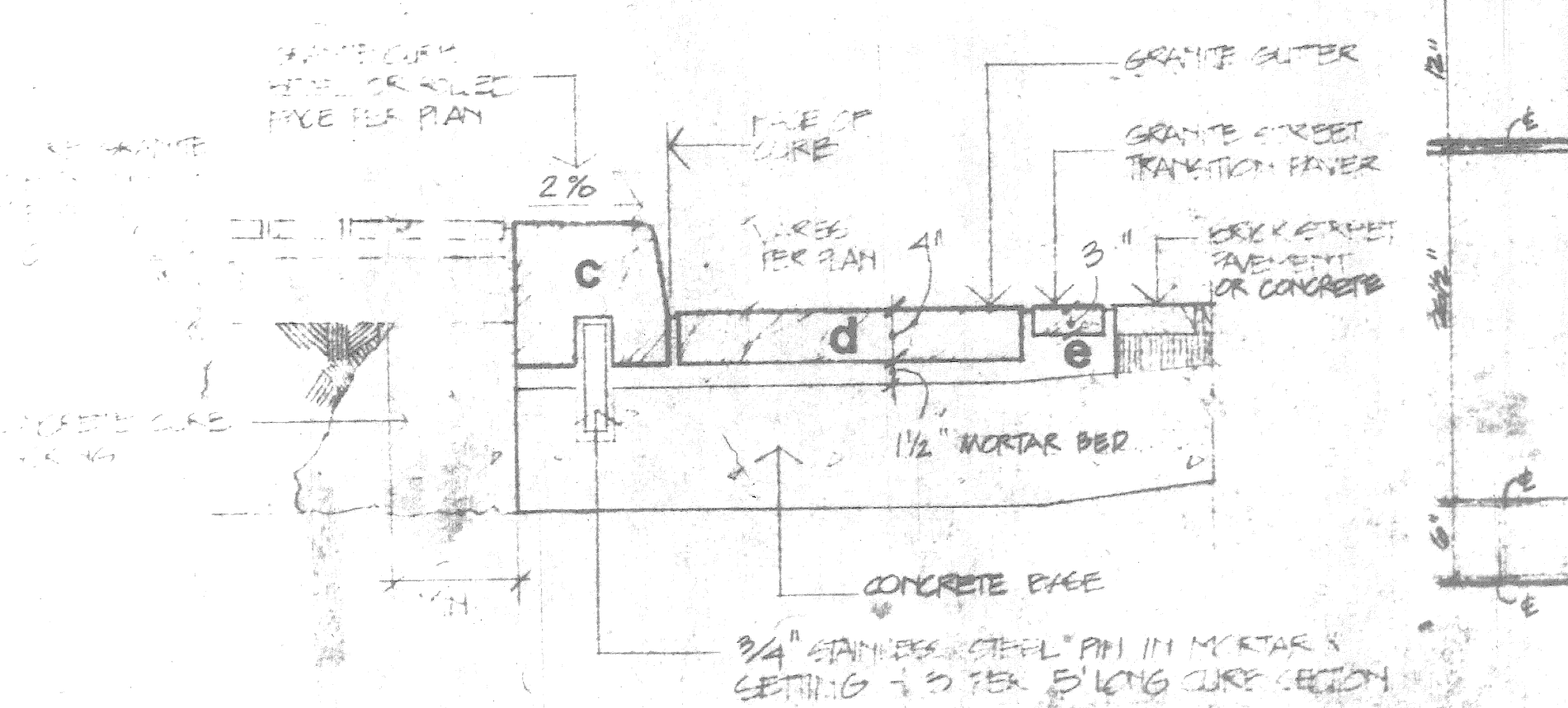
4 GRANITE PAVEMENT - STRAIGHT SEGMENT - SECTION 1" = 1'-0"
