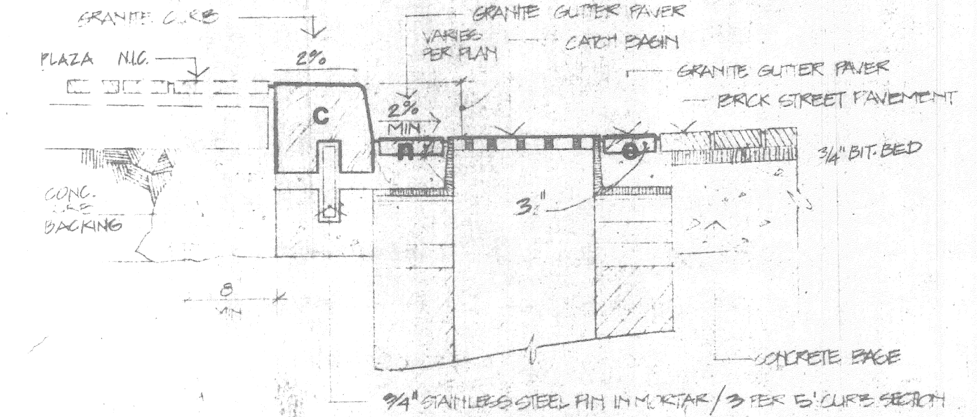
2 GRANITE PAVERS AT INLET - SECTION 1" = 1'-0"
