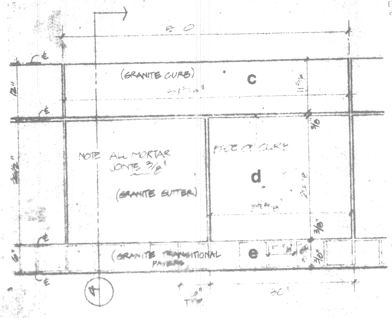
5 GRANITE PAVEMENT - STRAIGHT SEGMENT - LAYOUT 1" = 1'-0"
