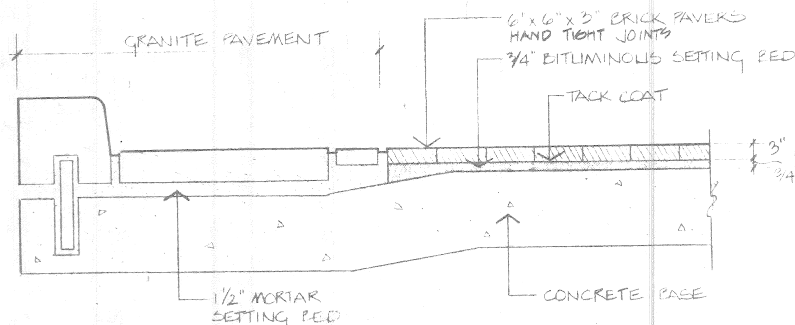
7 STREET BRICK SETTING BED SCALE 1" = 1'-0"
