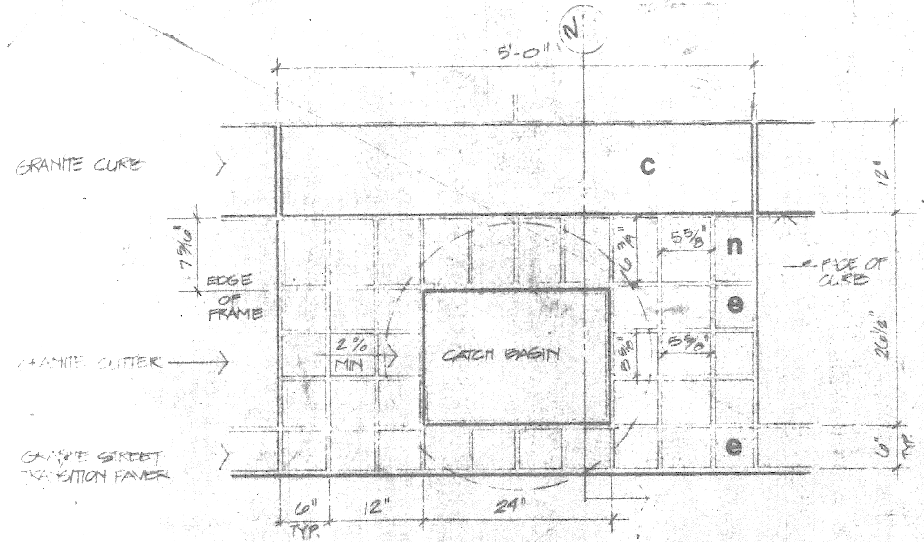
1 GRANITE PAVERS AT INLET - PLAN 1" = 1'-0"
