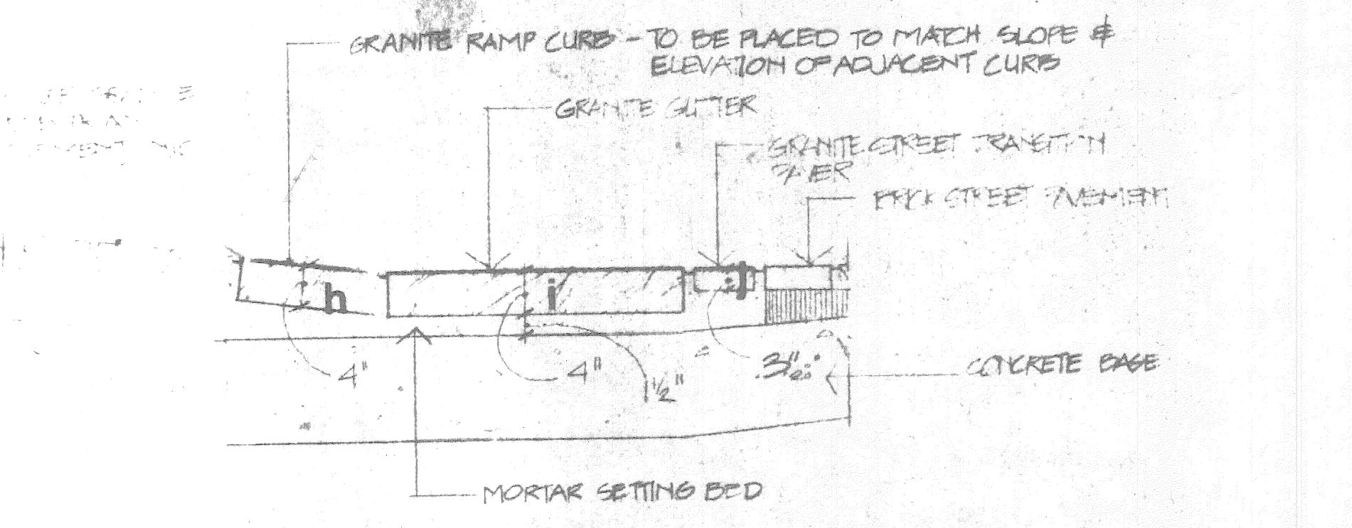
3 GRANITE PAVEMENT - DIAGONAL SEGMENT - SECTION 1" = 1'-0"
