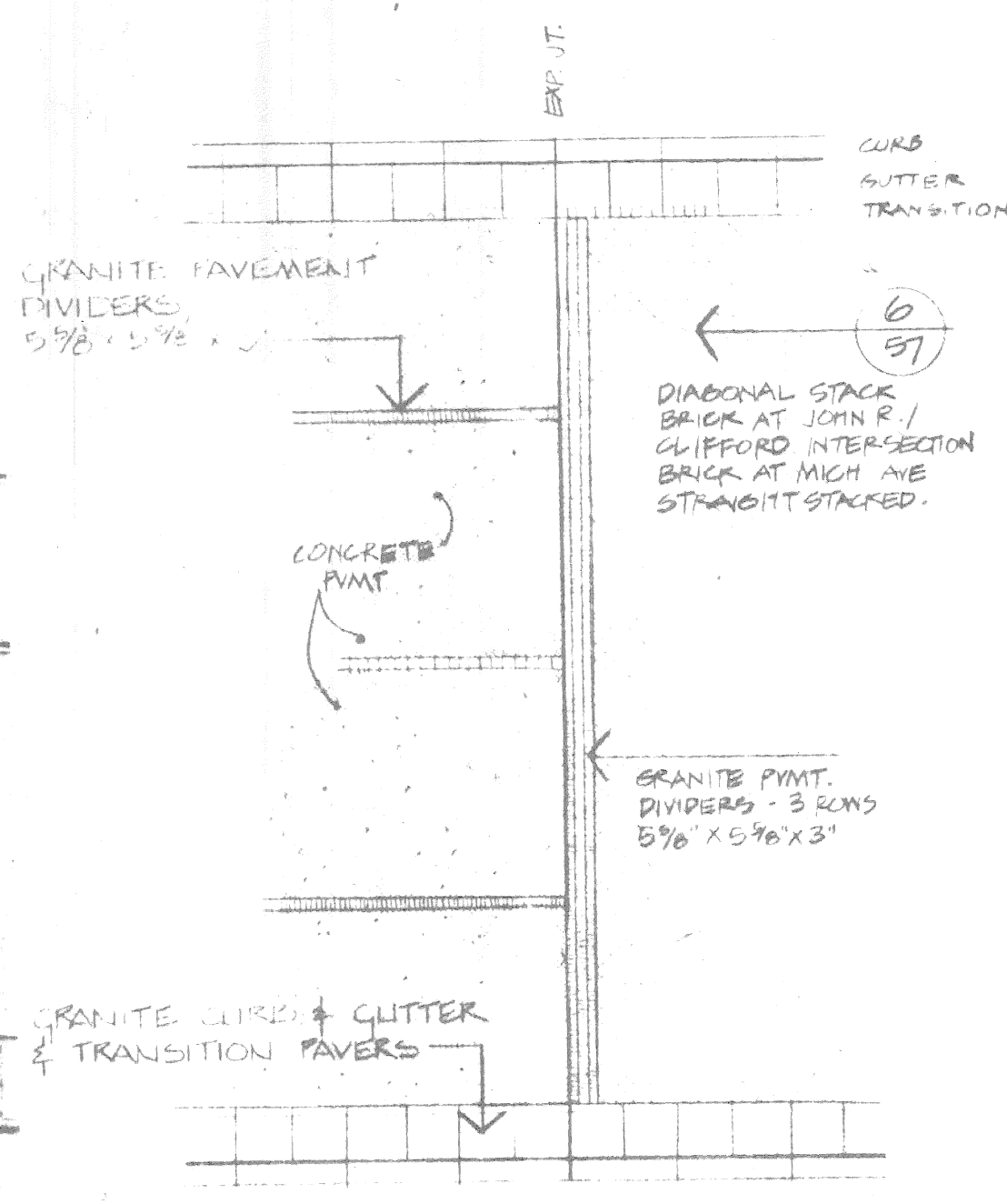
8 STREET PAVEMENT & DIVIDERS TYPICAL LAYOUT SCALE 1/8" = 1'-0"
