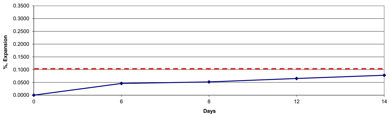
56% Coarse Aggregate / 44% Fine Aggregate / 0% Slag Cement
