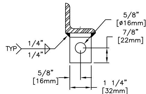
BOLT TAB DETAIL
