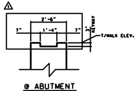
KEYWAY DETAILS
