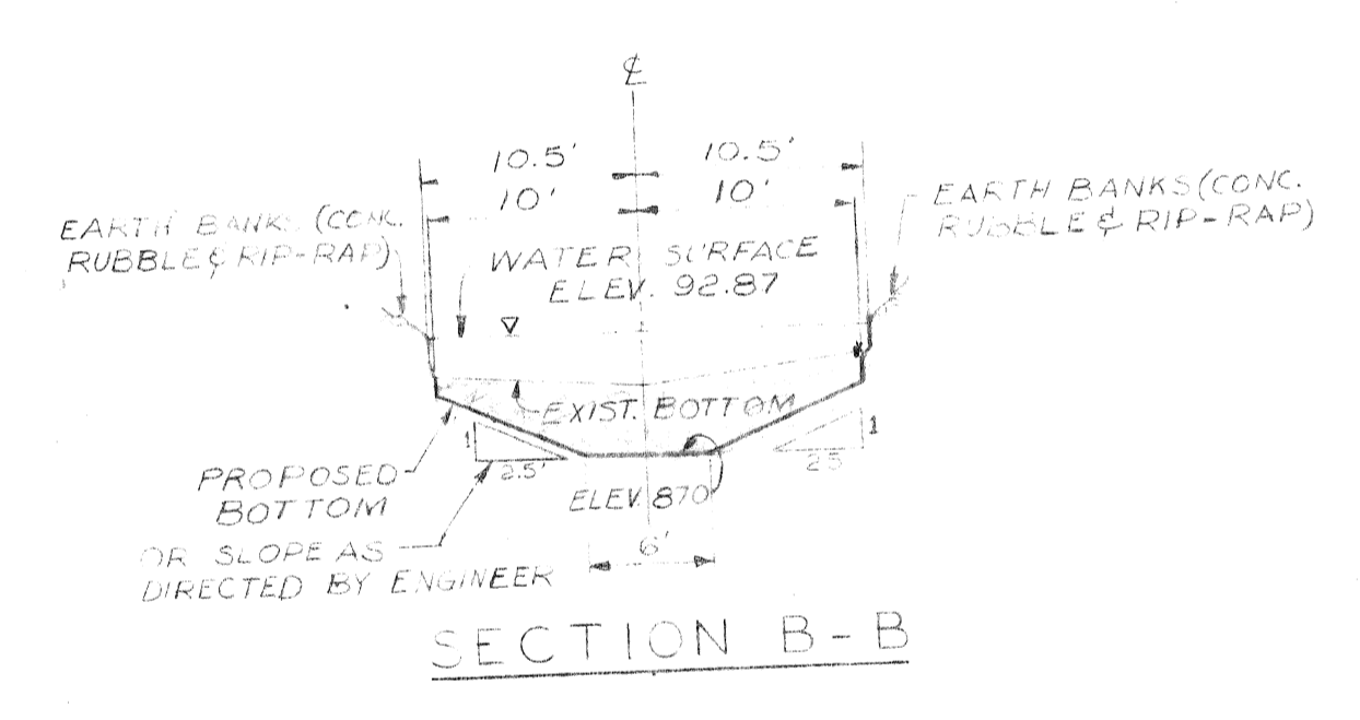
CROSS SECTIONS SCALE: HORZ. & VERT. 1"=10'
