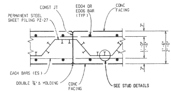
TYPICAL SECTION THRU CONC CAP (THE MIN. RED'D PLACEMENT OF STUDS PER ROW IS AS SHOWN) (SPACE ROWS @ 1'-6\"/>
