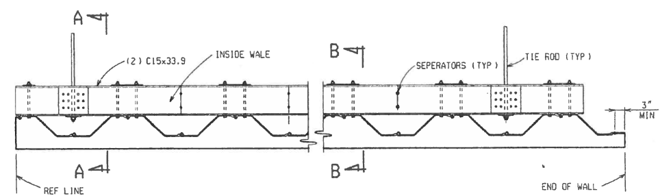
PLAN OF WALE AND TIE ROD (TYP. ALL WALLS)
