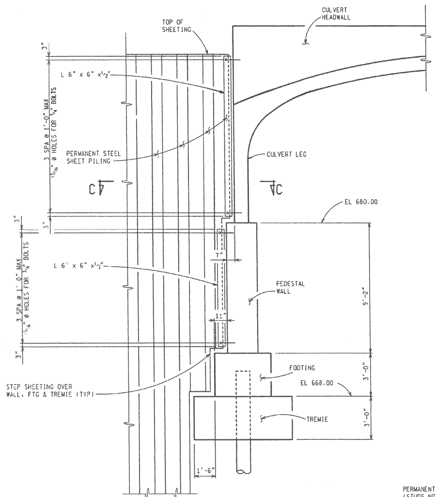
SECTION THRU PERMANENT SHEETING ANCHORAGE (TYP. ALL QUADRANTS)
