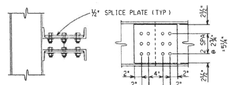
SPLICE PLATE OR STIFFENER PLATE DETAILS
