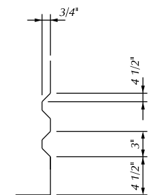
RUSTICATION DETAIL (SHOWING RUSTICATION)
