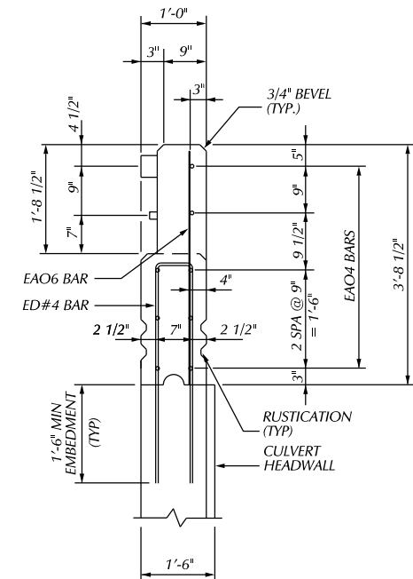
SECTION AT CULVERT END WALL (TUBE CONNECTION AREA)
