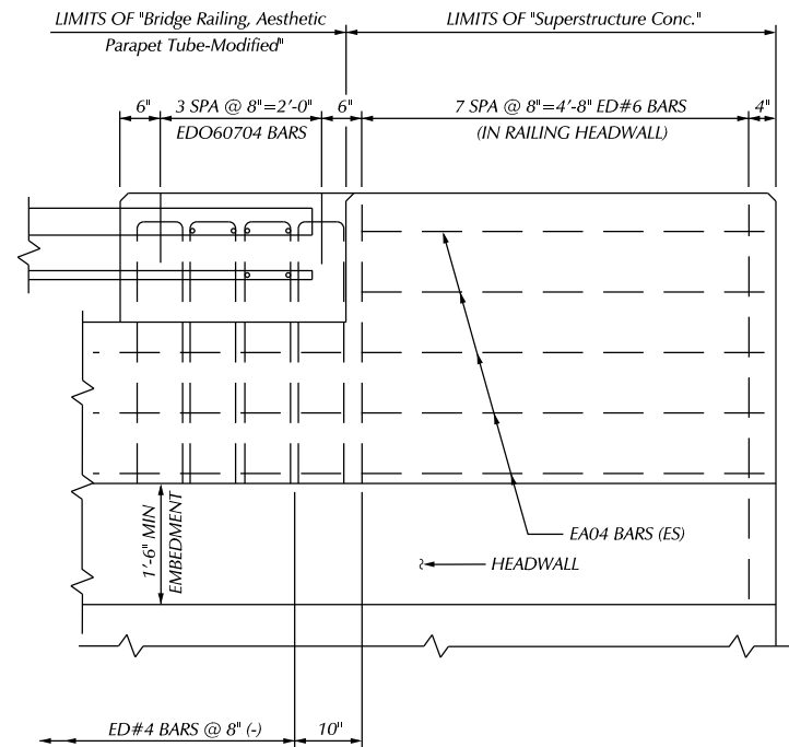
PLAN - CULVERT END WALL DETAIL
