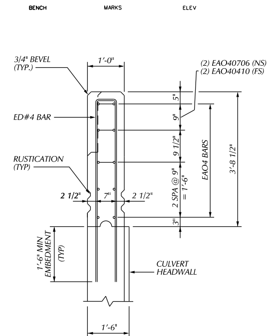
SECTION AT CULVERT END WALL (FULL CONCRETE AREA)
