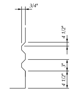
RUSTICATION DETAIL (SHOWING RUSTICATION)
