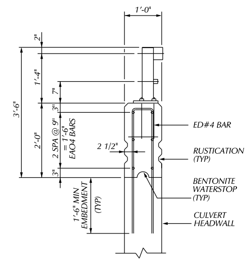
TYPICAL CULVERT RAILING SECTION
