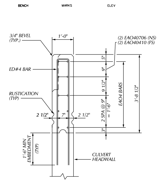
SECTION AT CULVERT END WALL (FULL CONCRETE AREA)
