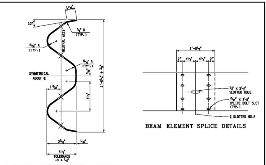
SECTION THROUGH BEAM ELEMENT
