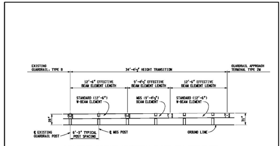
ELEVATION SHOWING TRANSITION DETAIL FOR CONNECTING GUARDRAIL, TYPE B TO GUARDRAIL APPROACH TERMINAL TYPE 2M
