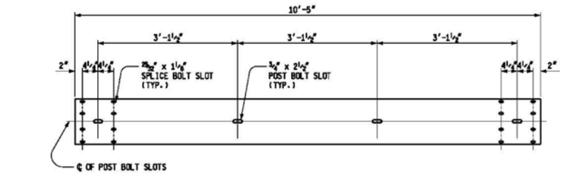
FRONT ELEVATION OF MGS (9'-4 1/2") BEAM ELEMENT
