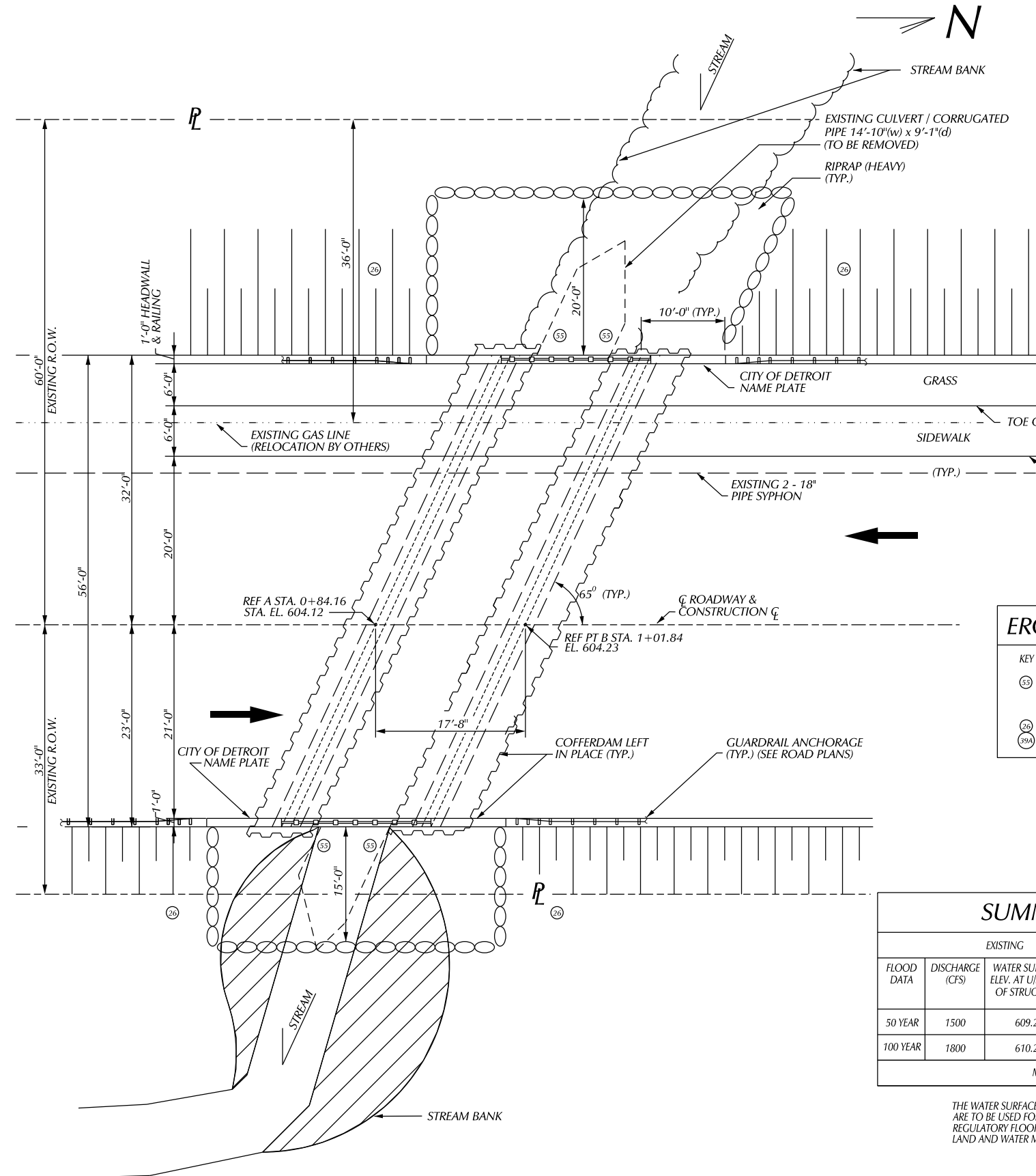
PLAN
