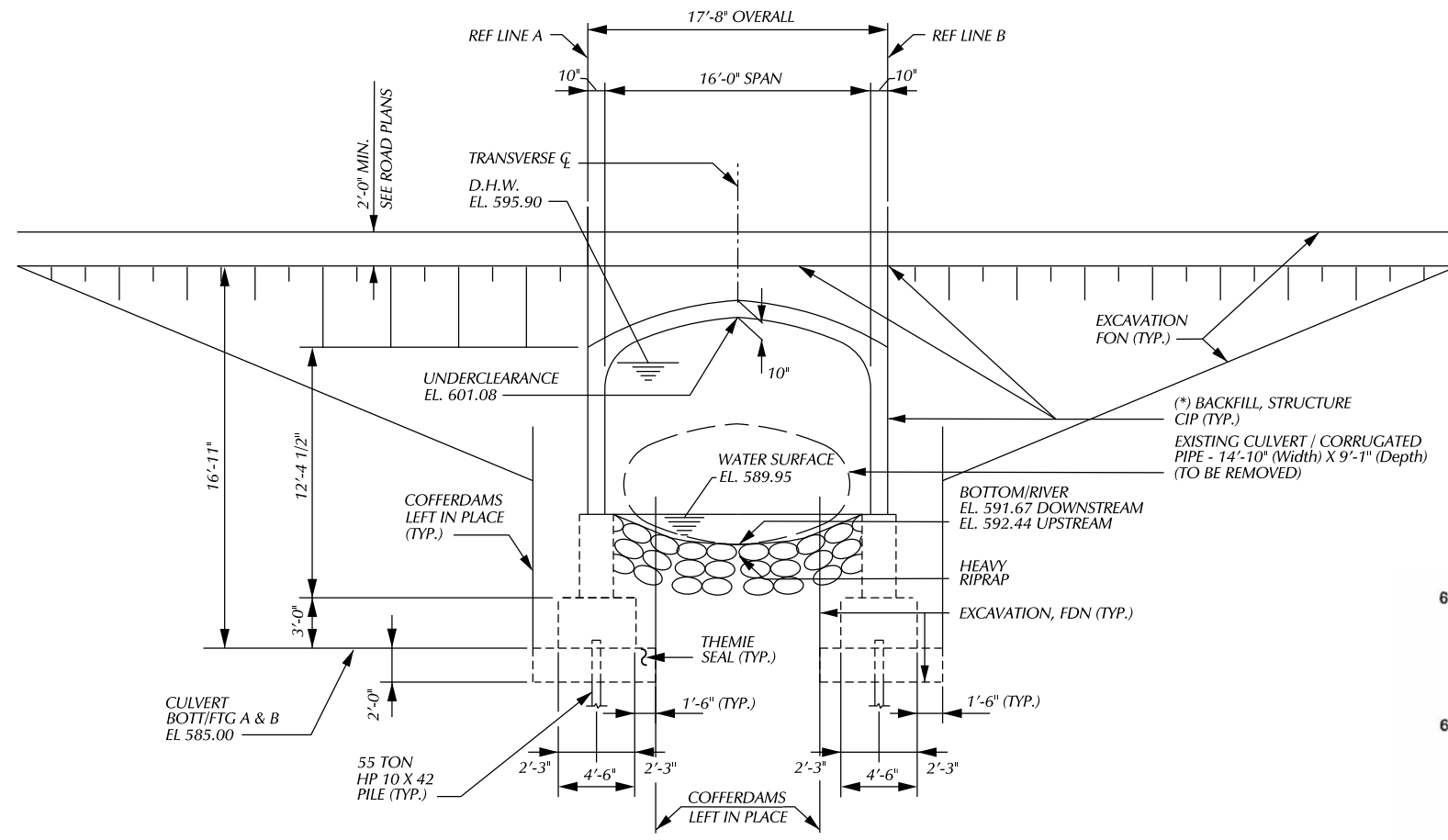
CULVERT SECTION
