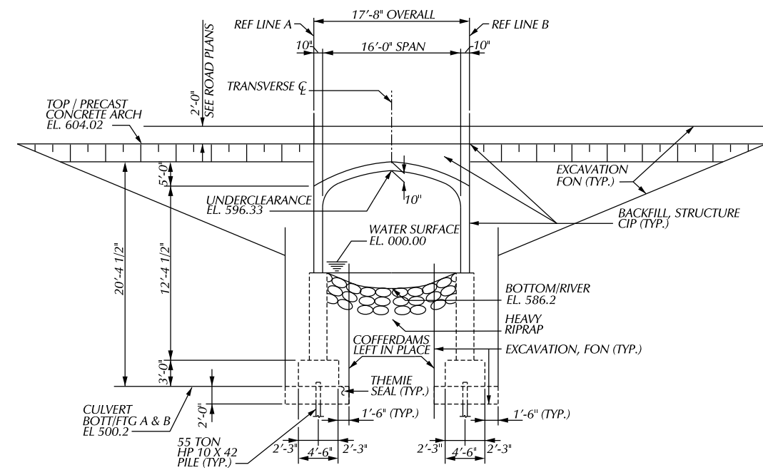
CULVERT SECTION
