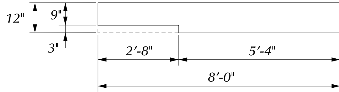
PLAN - CULVERT END WALL
