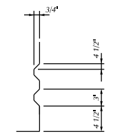
RUSTICATION DETAIL (SHOWING RUSTICATION)
